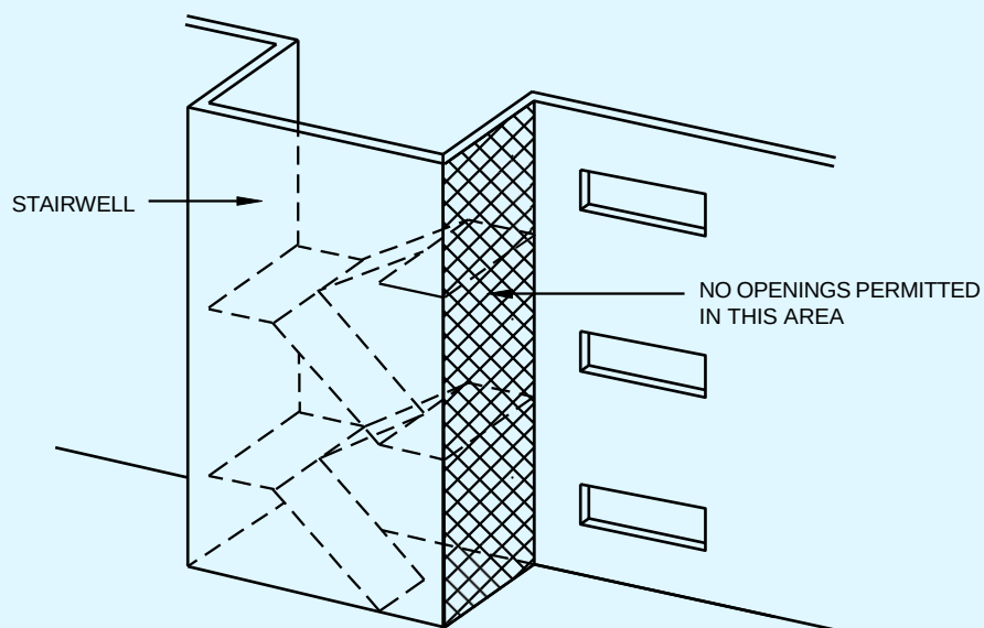
14A LIMITATIONS ON OPENINGS NEAR STAIRWELL
