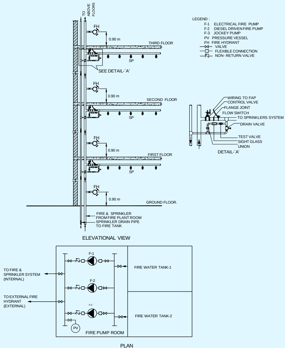
FIG. 15 TYPICAL SYSTEM OF PUMPING WITH ONE ELECTRIC, ONE DIESEL FIRE PUMP
