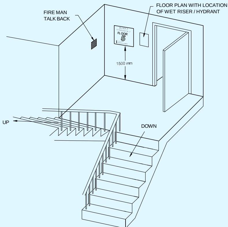
9B STAIR SIGN PLACEMENT
