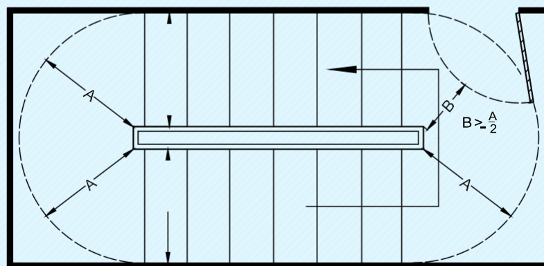
7B MINIMUM REQUIRED UNOBSTRUCTED CLEARANCE WITH DOOR LEAF ENCROACHING ON LANDING
