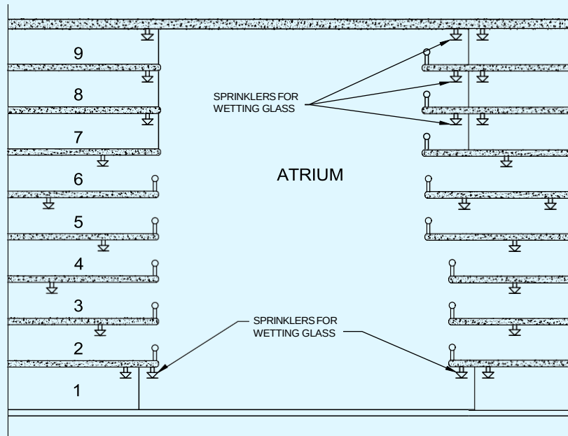
FIG. 22 SPRINKLER PROTECTION OF GLASS FOR FLOOR OPEN TO ATRIUM
